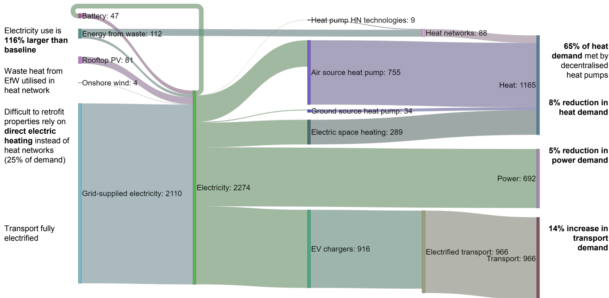
Figure 3.3: Energy flows (GWh/year) in Dundee's High Electrification scenario
