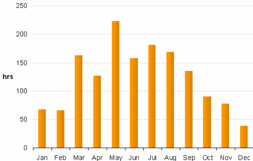
Chart 35: Monthly sunshine totals 2009
