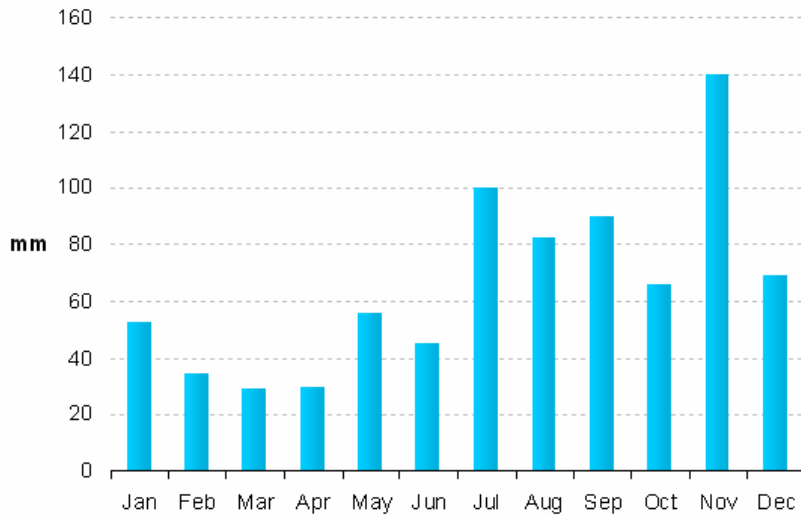
Chart 34: Monthly rainfall totals 2009
