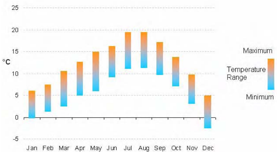
Chart 33: Monthly average maximum and minimum temperatures for 2009
